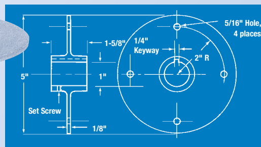
Heavy Duty Sprocket Holder/Hub
